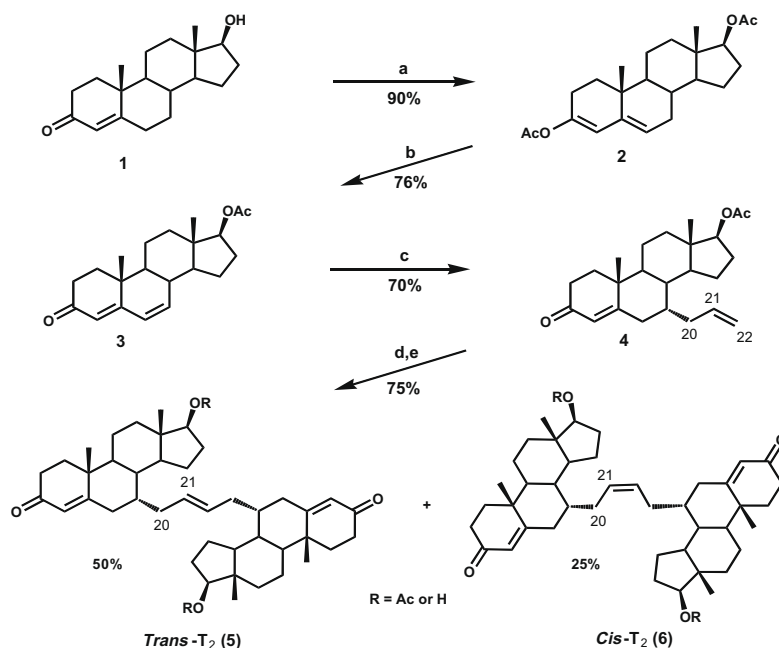
Scheme 1. Reagents and conditions: (a) AcCl, Ac 2 O, Pyr, reflux, 4 h; (b) (1) NBS, DMF, 0 °C, 1.5 h, (2) Li 2 CO 3 , LiBr, DMF, 92 °C, 4 h; (c) (1) TiCl 4 , Pyr, DCM, −78 °C, 5 min, (2) allyltrimethylsilane, −30 °C, 1.5 h; (d) Hoveyda–Grubb's catalyst 2nd generation, CH 2 Cl 2 (75%); (e) 10% aqueous HCl, MeOH, (95%).
