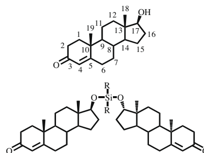
Figure 1. Testosterone structure and known testosterone dimers (R = Me or Ph).
