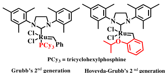
Figure 3. Catalysts used for the Grubb's metathesis.
